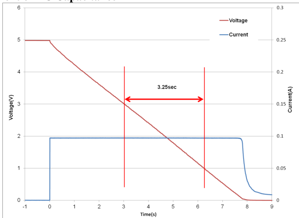
Fig 2: Measurement of DC Capacitance for an HW209
