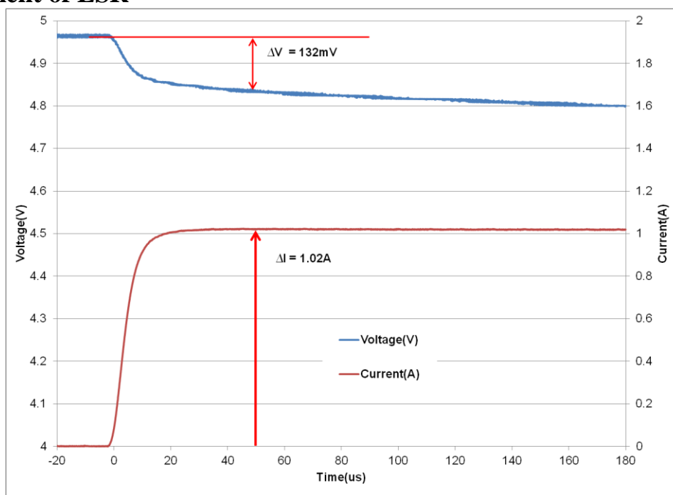
Fig 3: Measurement of ESR for an HW209
