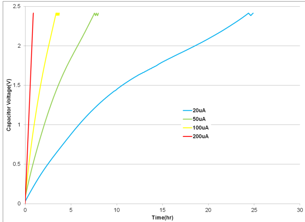
Fig 11: Charging an HW109 with low current
