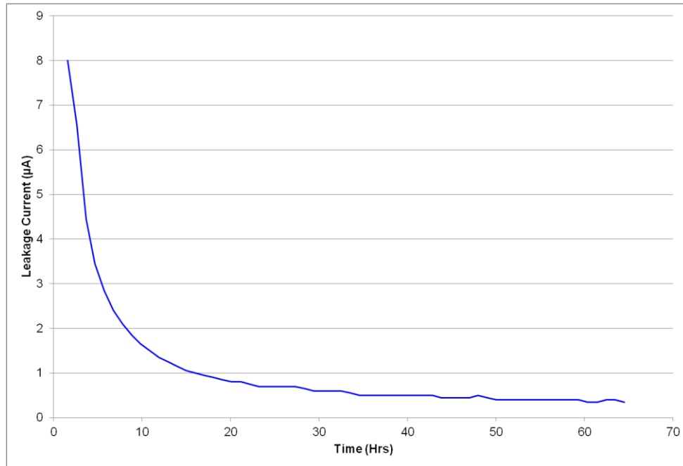
Fig 10: Leakage Current
