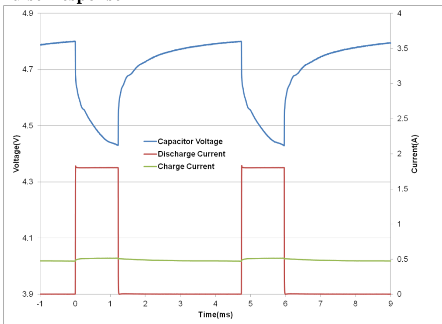
Fig 5: HW209 Pulse Response with GPRS Class 10 Pulse Train
