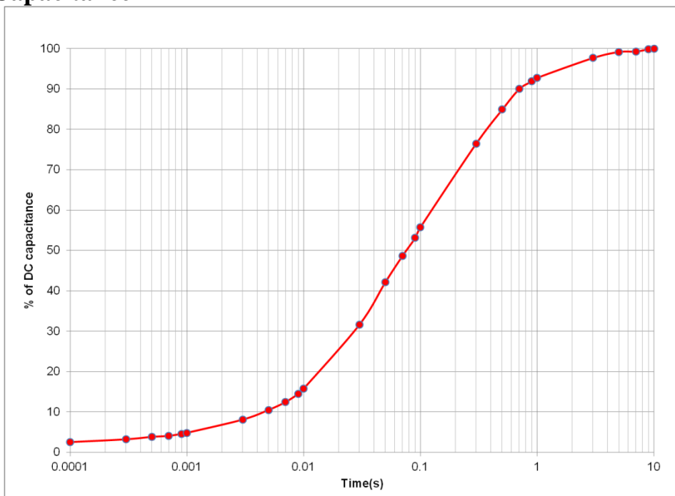
Figure 4: Effective Capacitance
