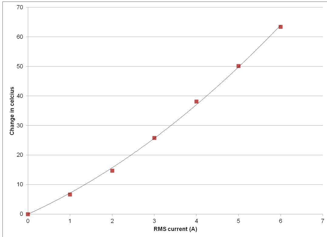
Fig 12: Temperature rise in HW209 with RMS current
